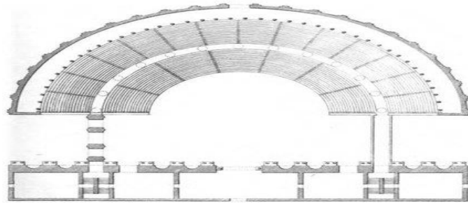
PLAN OF THE LARGER THEATRE AT GORTYNA.
