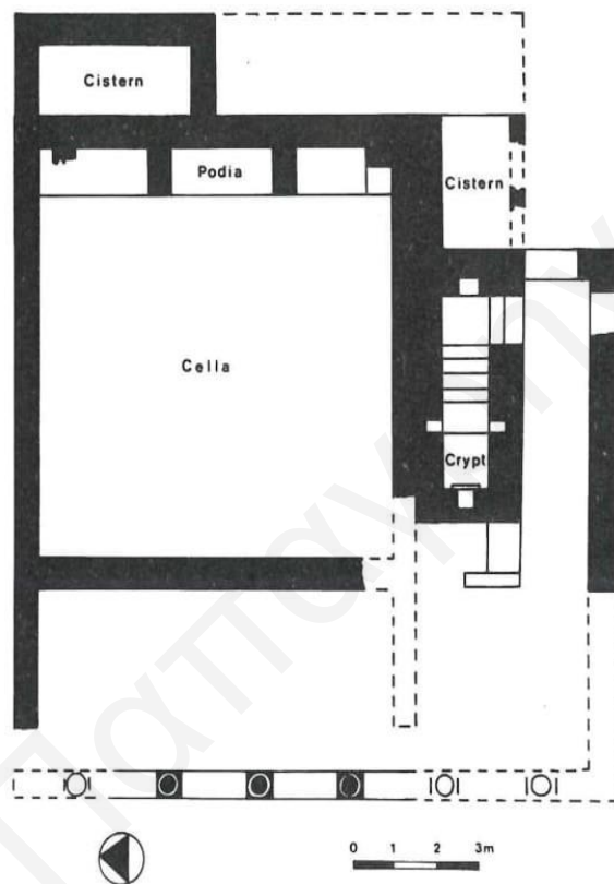
Fig.15. Gortyna: plan of the temple of Isis and Serapis.
