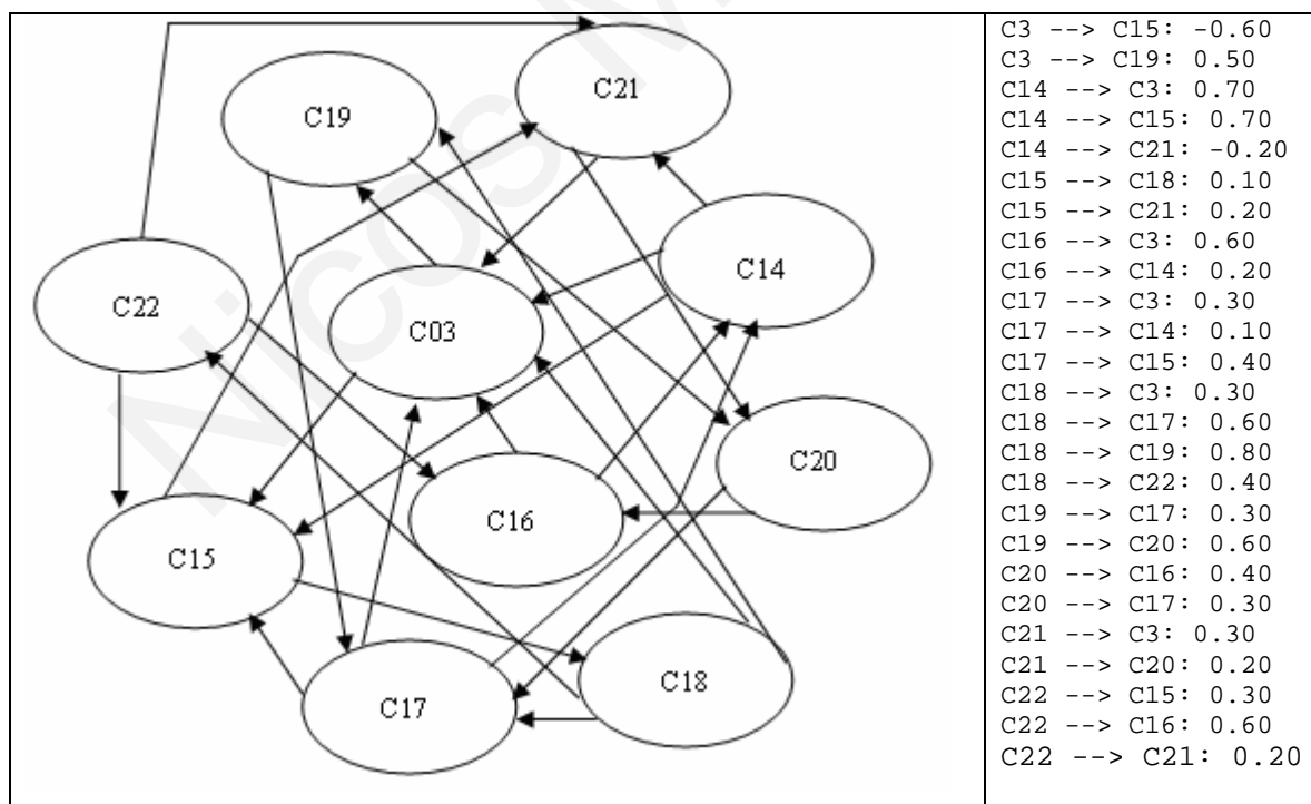
Figure 5.7: FCM2 expanded representation
