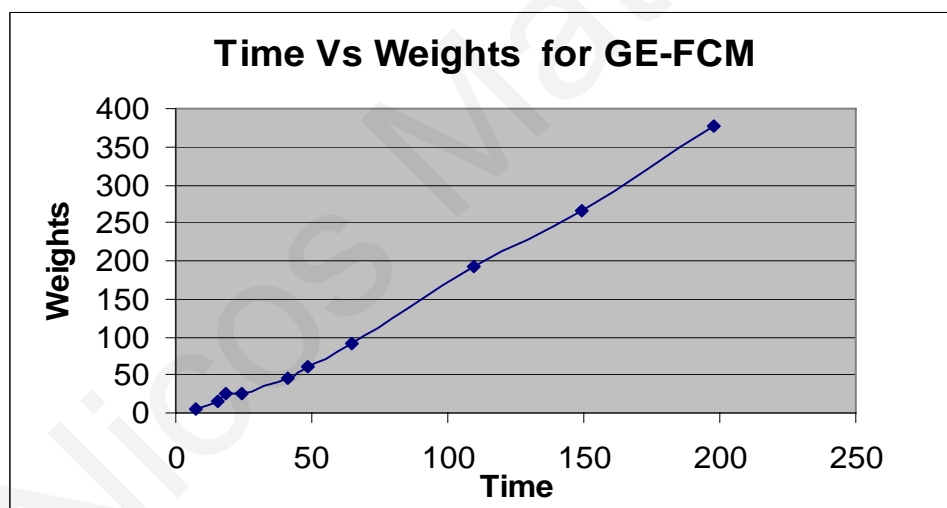
Figure 4.32: Graphical representation of time performance with respect to weights for the GE-FCM
