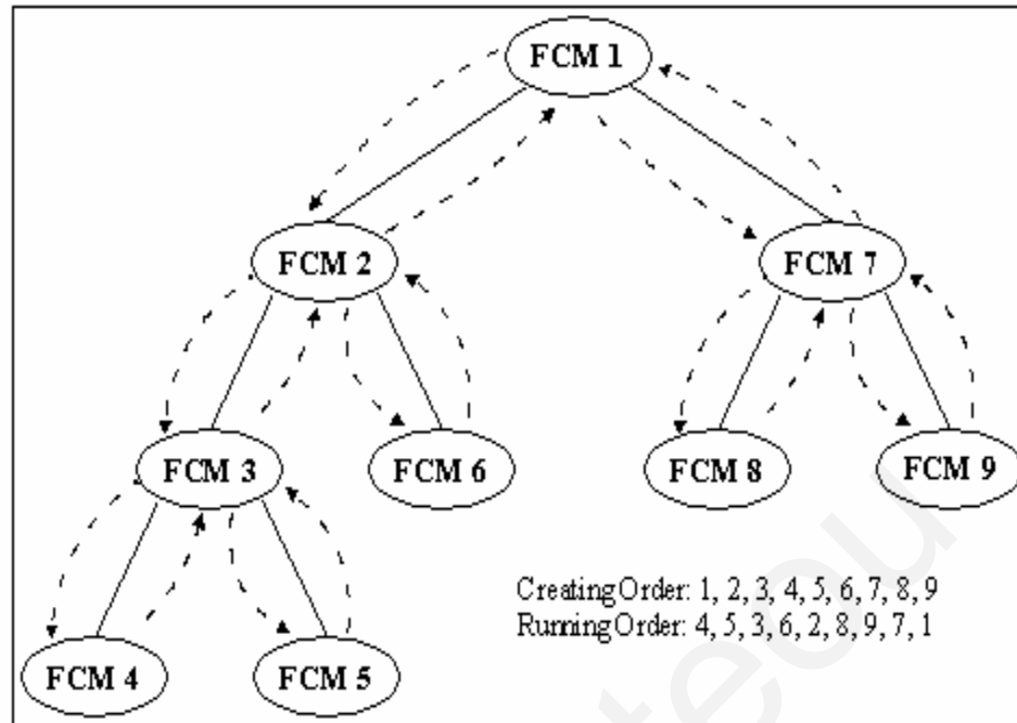
Figure 5.3: An example of a ML-FCM
