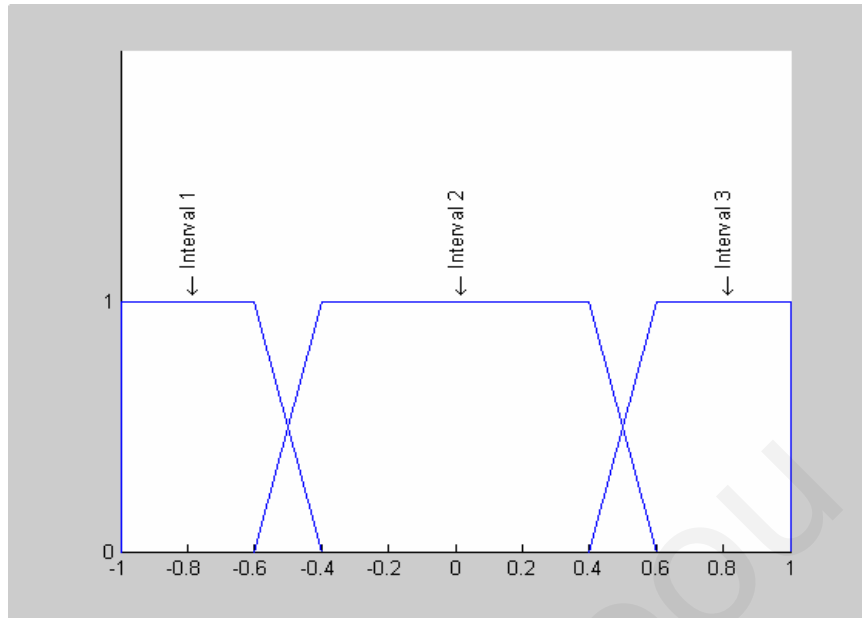
Figure 2.7: Parameter with 3 membership functions of variable width
