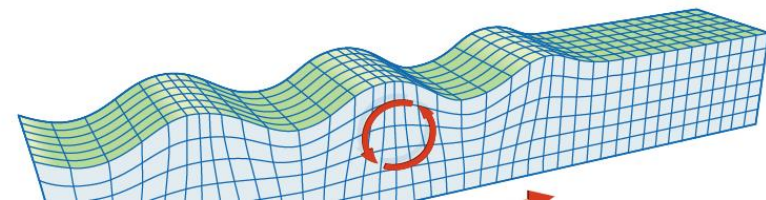
Rayleigh wave
