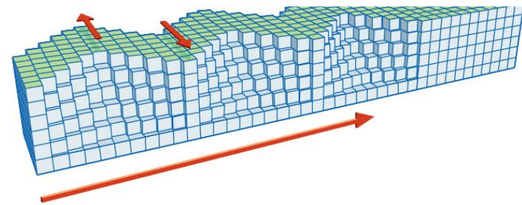
Rayleigh wave
