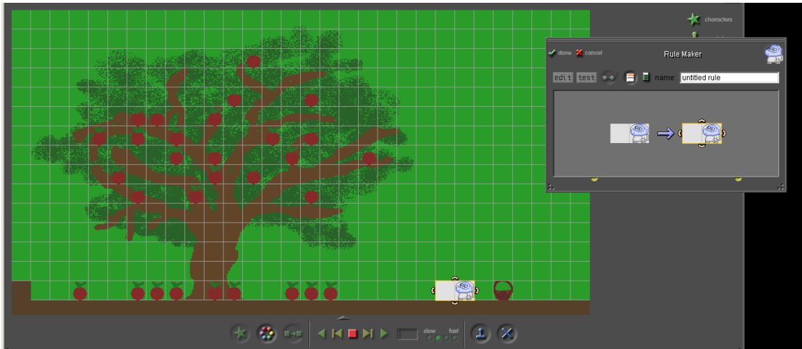
Figure 2. The interface of Stagecast Creator™: applying rules to a character
