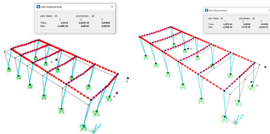
Fig. 7. Deformations of elastic modal analysis in the Ex (left) and Ey (right) application of loads.
