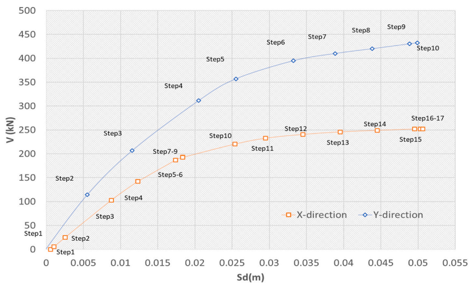
Fig. 9. Pushover curves in the X and Y direction.
