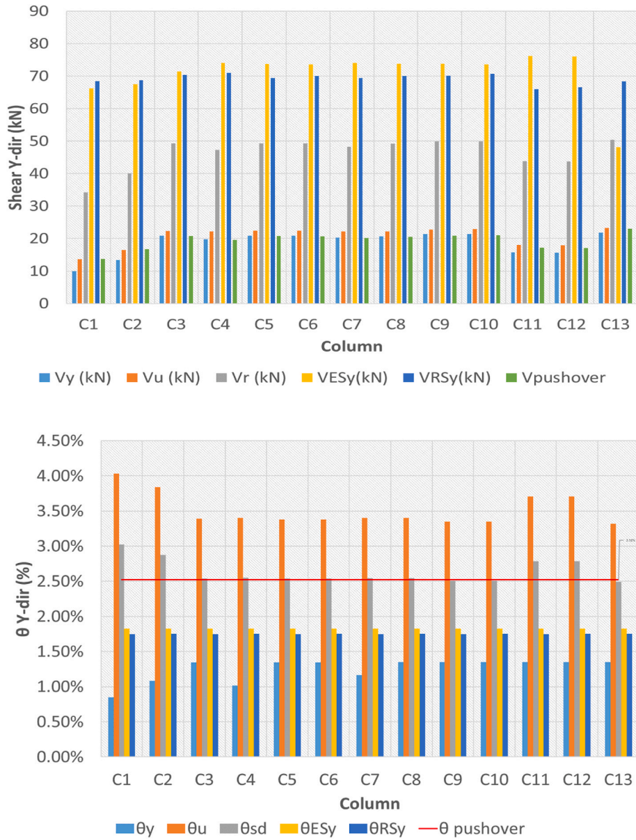
Fig. 10. Shear demand and capacity (top) and chord rotation demand and capacity (bottom).
