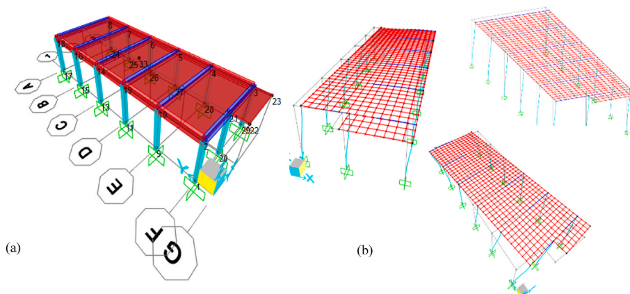
Fig. 5. (a) Model of the structure, (b) 1st, 2nd and 3rd mode shapes.
