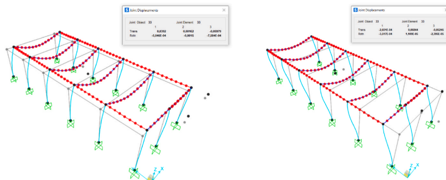
Fig. 6. Deformations of elastic static analysis in the Ex (left) and Ey (right) application of loads.
