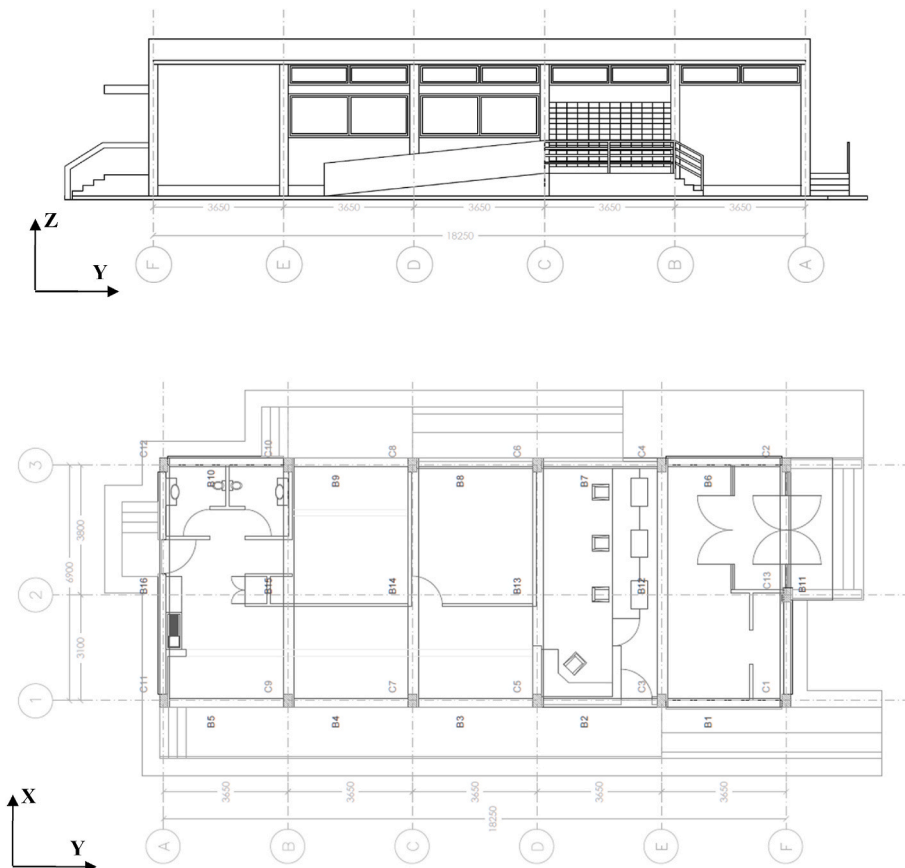
Fig. 2. Side (top) and Plan (bottom) view of the Pedieos Post Office.
