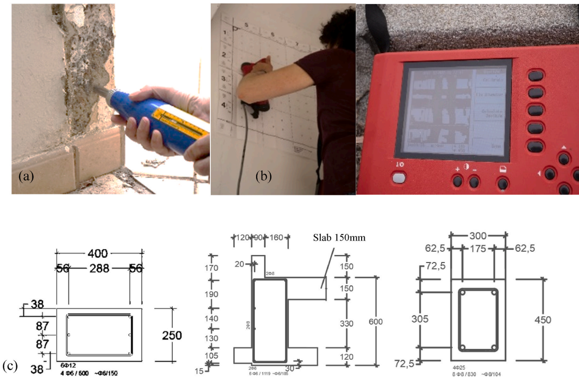
Fig. 4. (a) Schmidt rebound hammer test on column, (b) rebar detector, (c) column and beams detailing.
