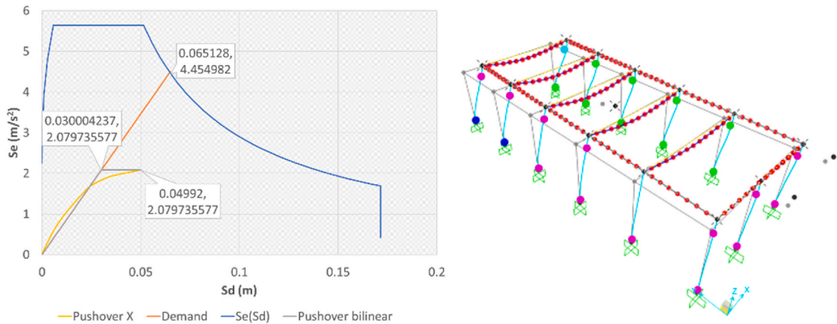
Fig. 11. Pushover curve and seismic demand (left) and formation of plastic hinges at the end of pushover (right) for the X direction.
