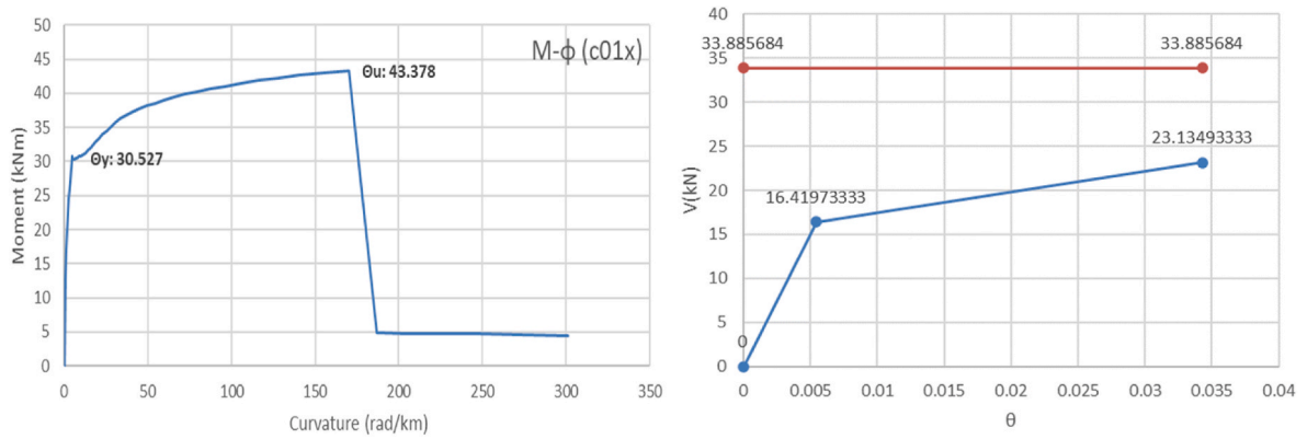
Fig. 8. Moment-curvature (left) and Shear-drift (right) for column K1 in the X-direction.
